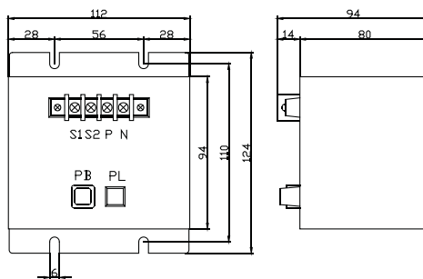
Dimensions & fixing holes of CTD
