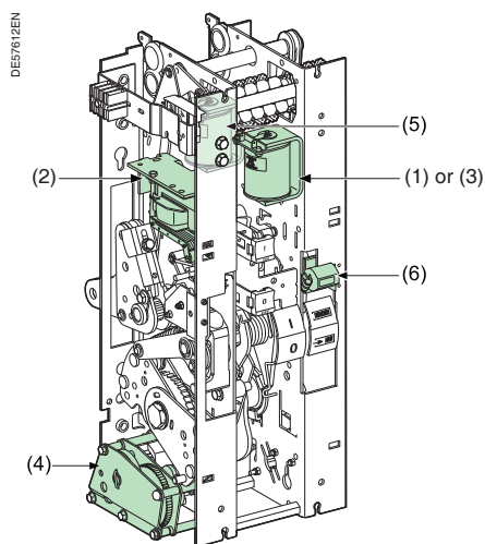
Operating mechanism
